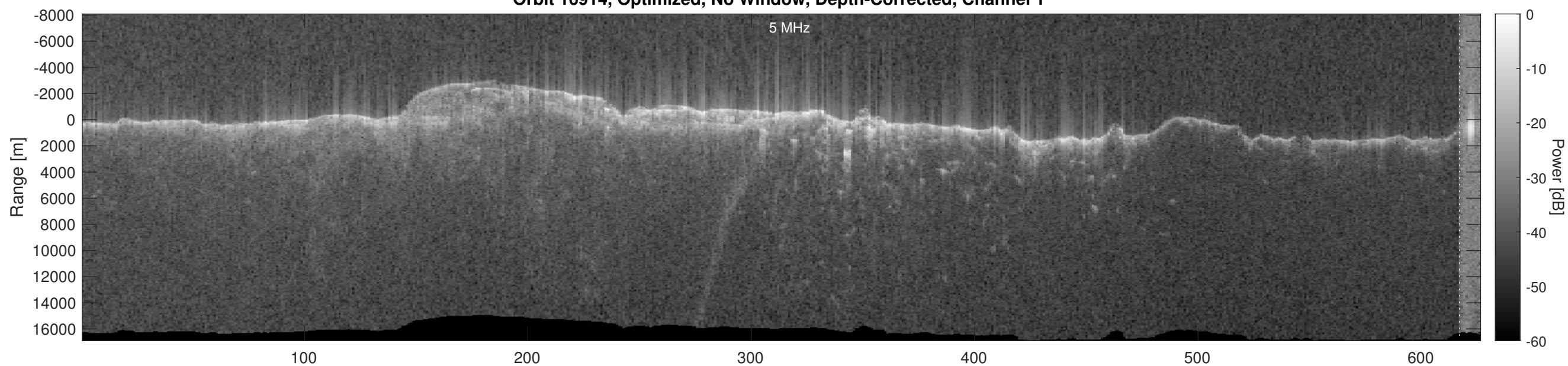
Orbit 16914, Optimized, No Window, Depth-Corrected, Channel 2
