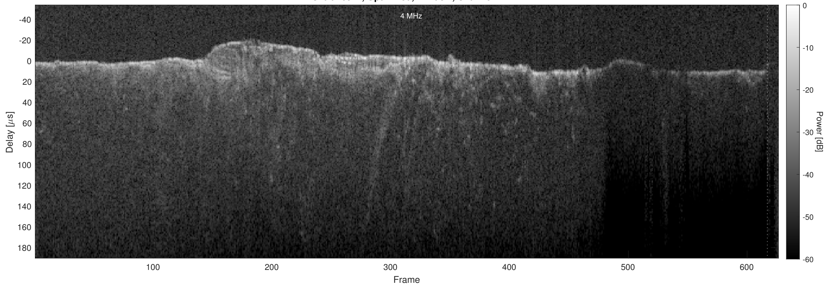
Orbit 16914, Optimized, Window, Channel 2
