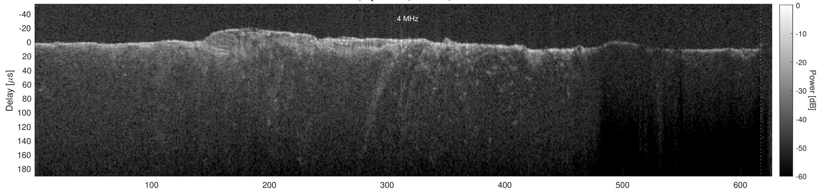
Orbit 16914, Cluttergram
