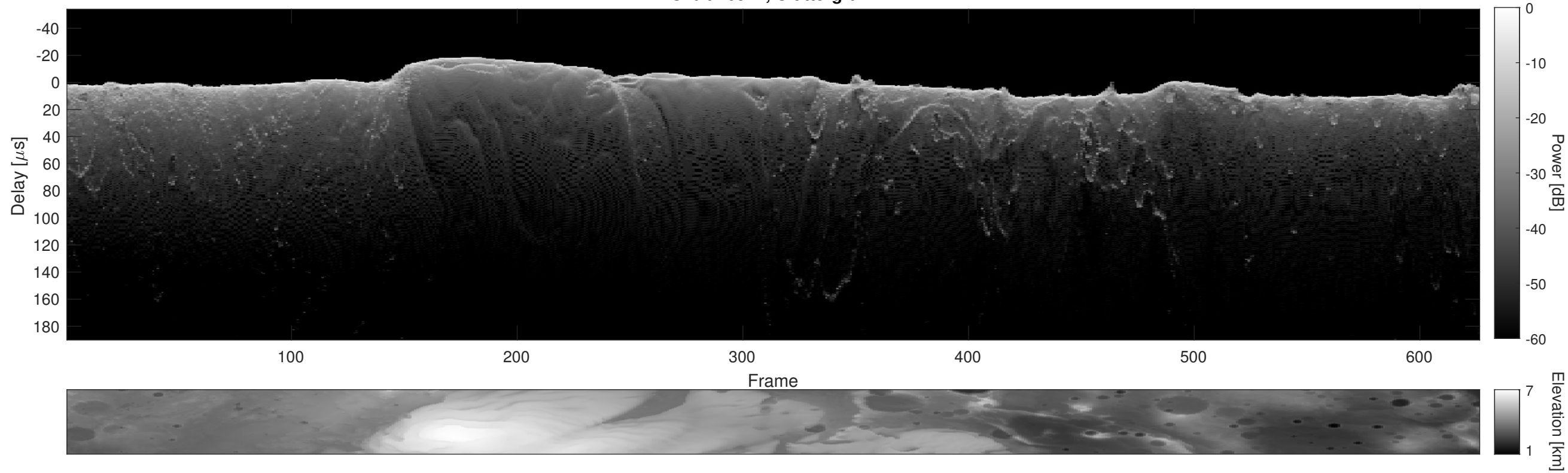
Orbit 16914, Cluttergram
