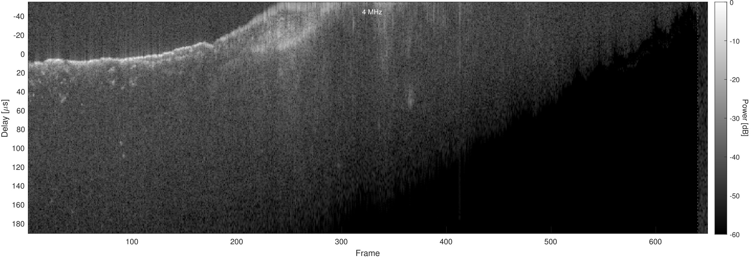
Orbit 16922, Chapman, No Window, Channel 2
