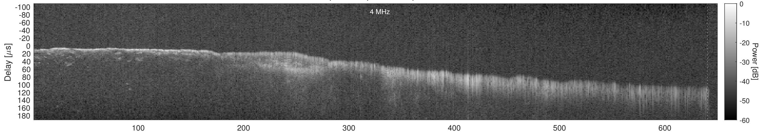
Orbit 16922, Window, Channel 2, Chapman
