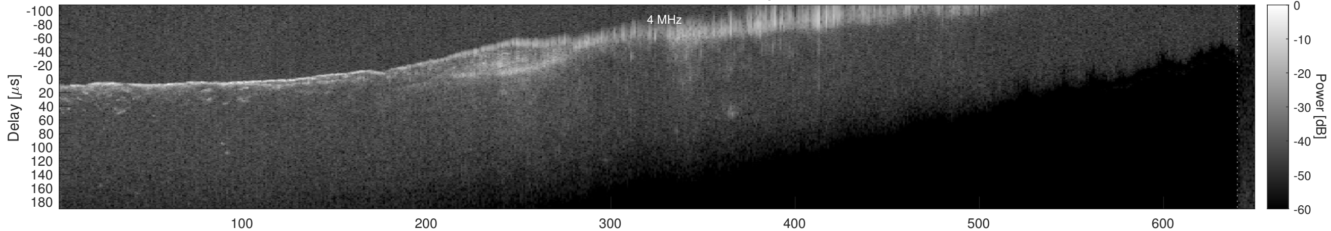
Orbit 16922, Window, Channel 2, Optimized
