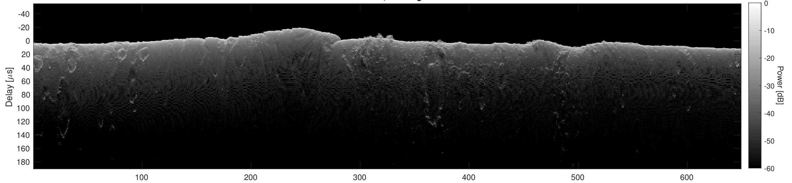
Orbit 16922, Cluttergram
