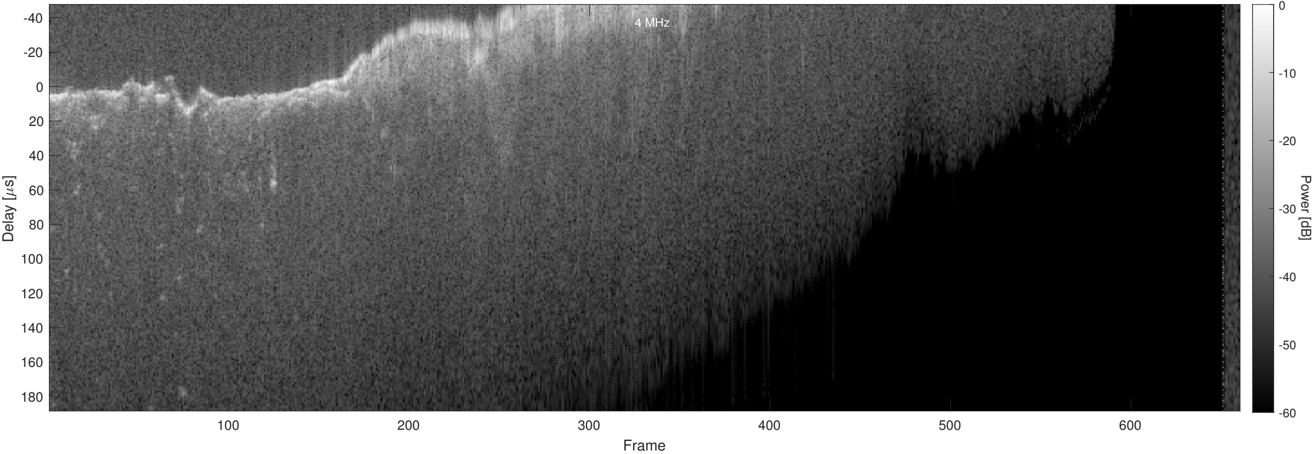
Orbit 16927, Chapman, No Window, Channel 2
