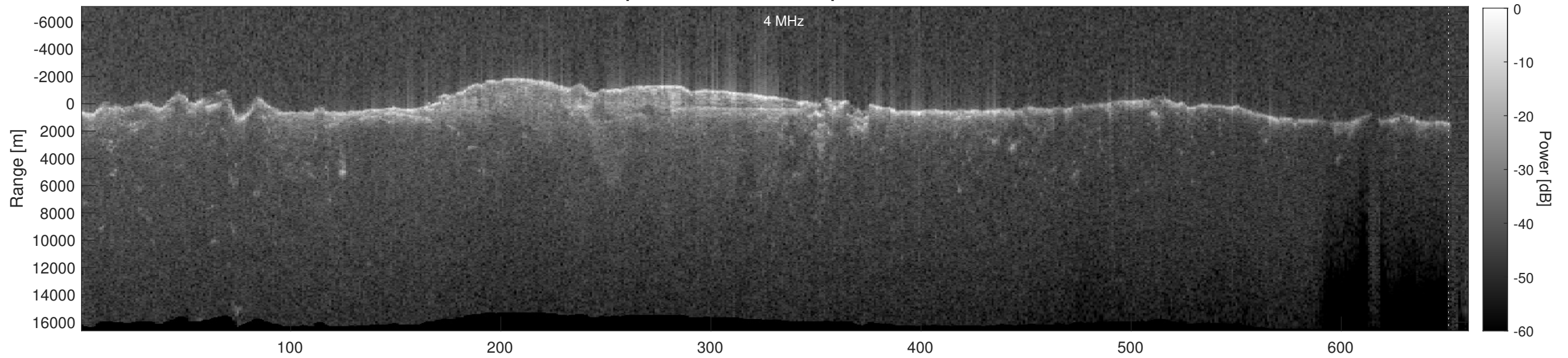
Orbit 16927, Depth-Corrected Cluttergram
