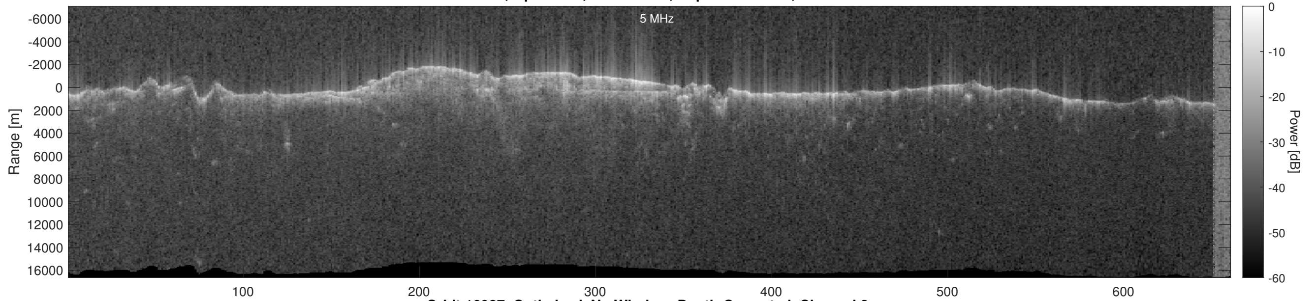
Orbit 16927, Optimized, No Window, Depth-Corrected, Channel 2
