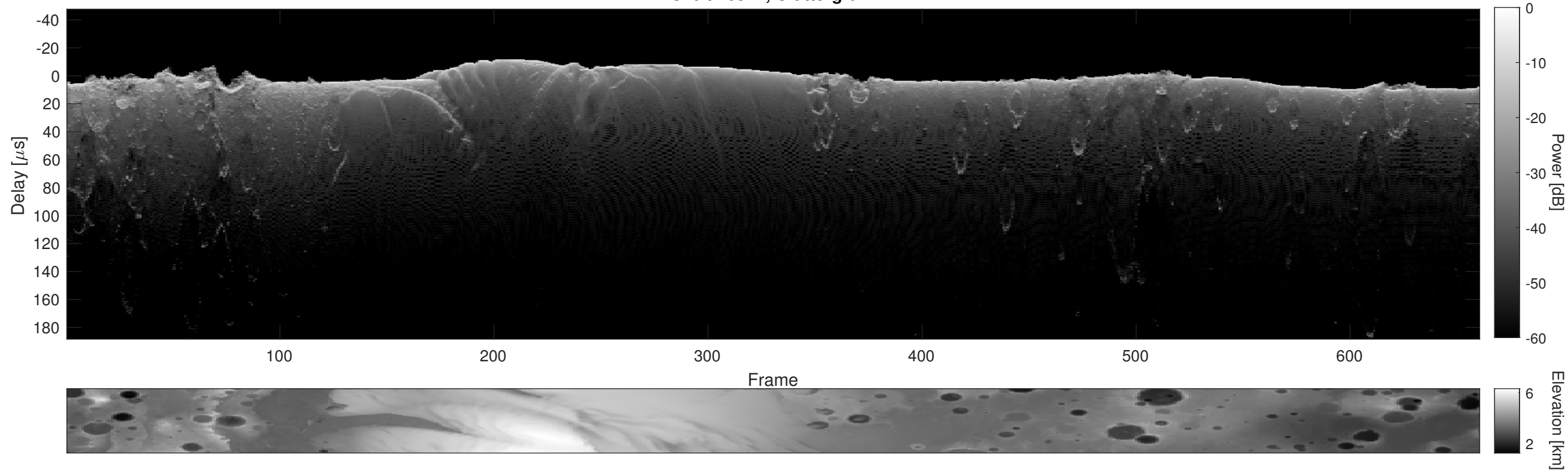
Orbit 16927, Cluttergram
