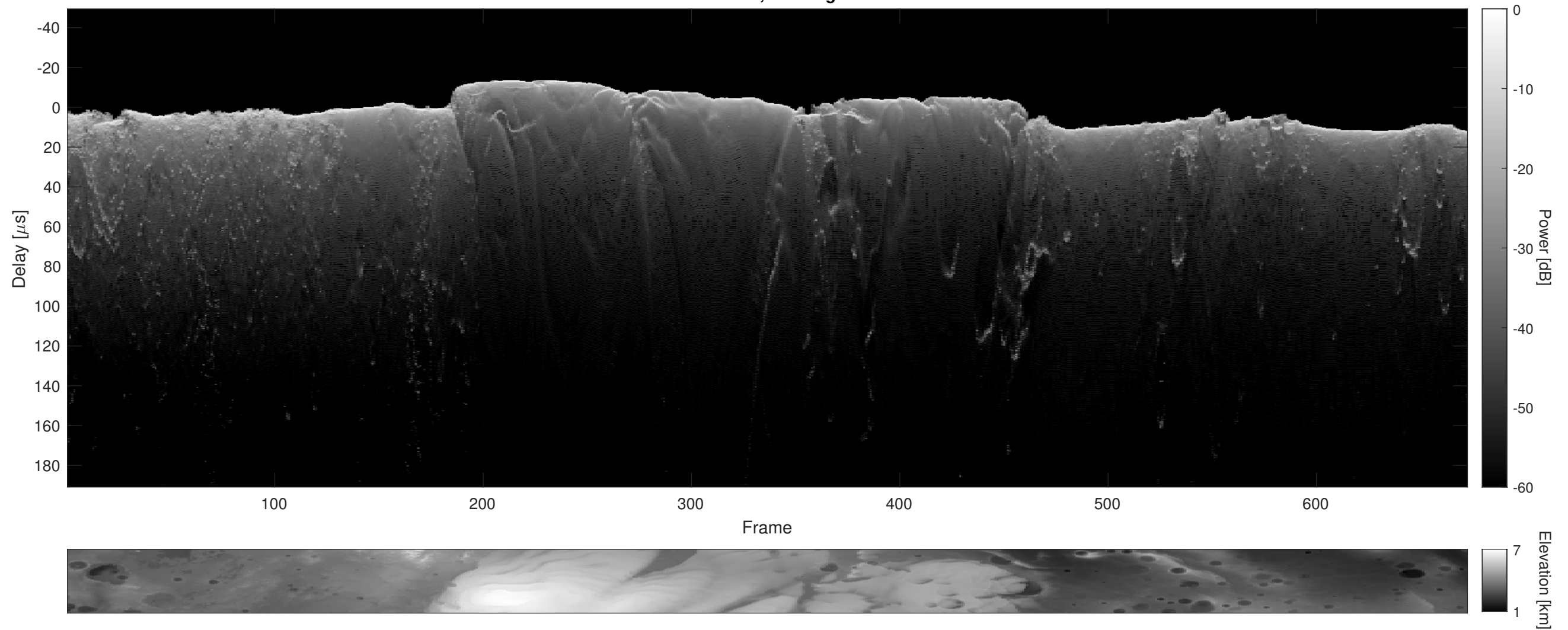
Orbit 16935, Cluttergram
