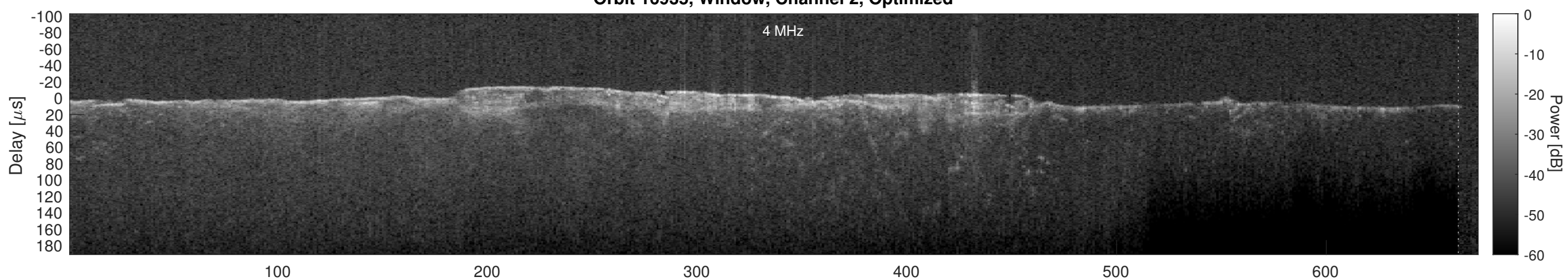
Orbit 16935, Cluttergram
