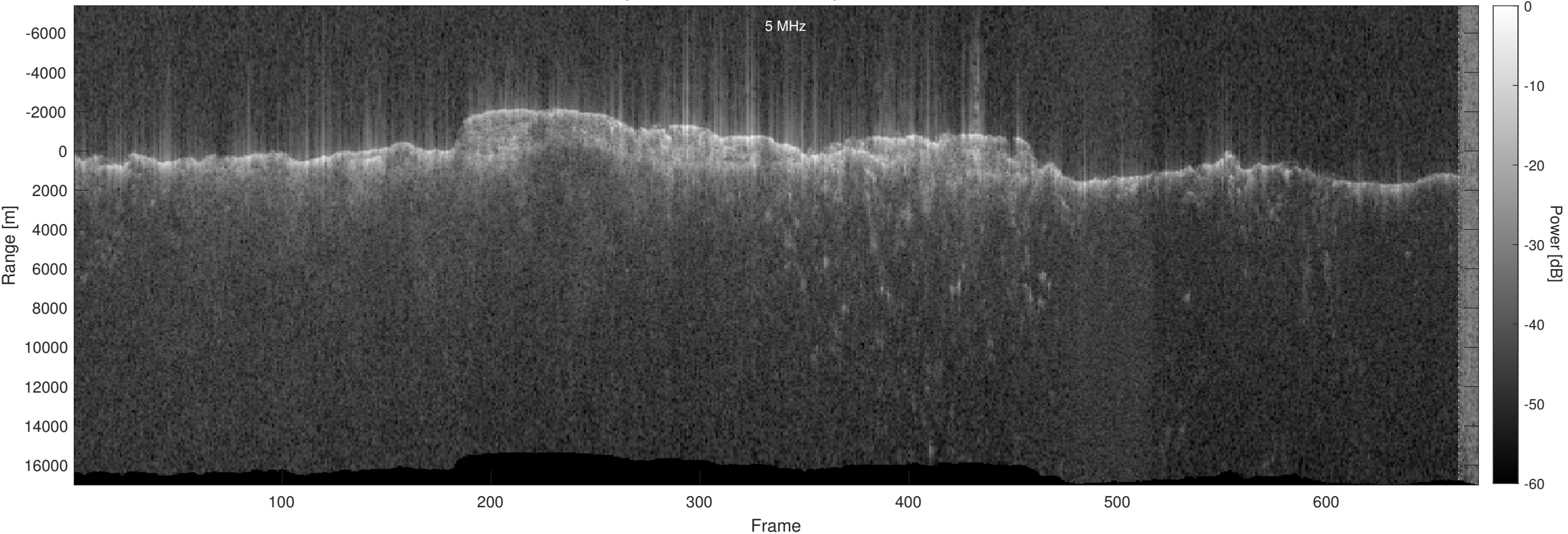
Orbit 16935, Optimized, No Window, Depth-Corrected, Channel 2
