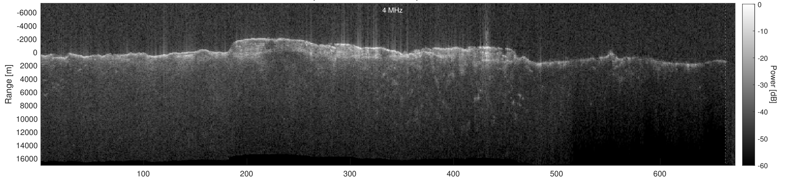
Orbit 16935, Depth-Corrected Cluttergram
