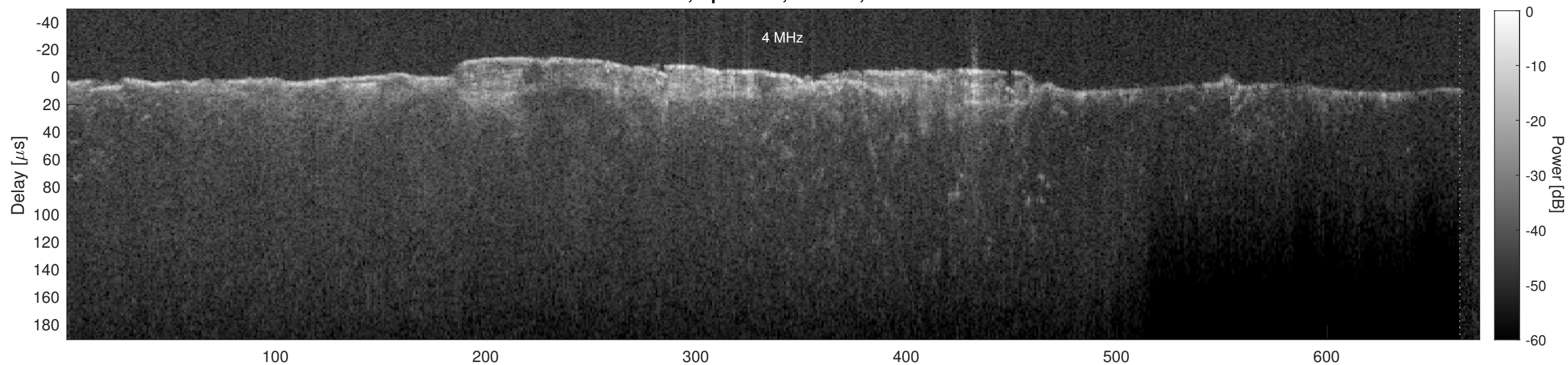
Orbit 16935, Cluttergram
