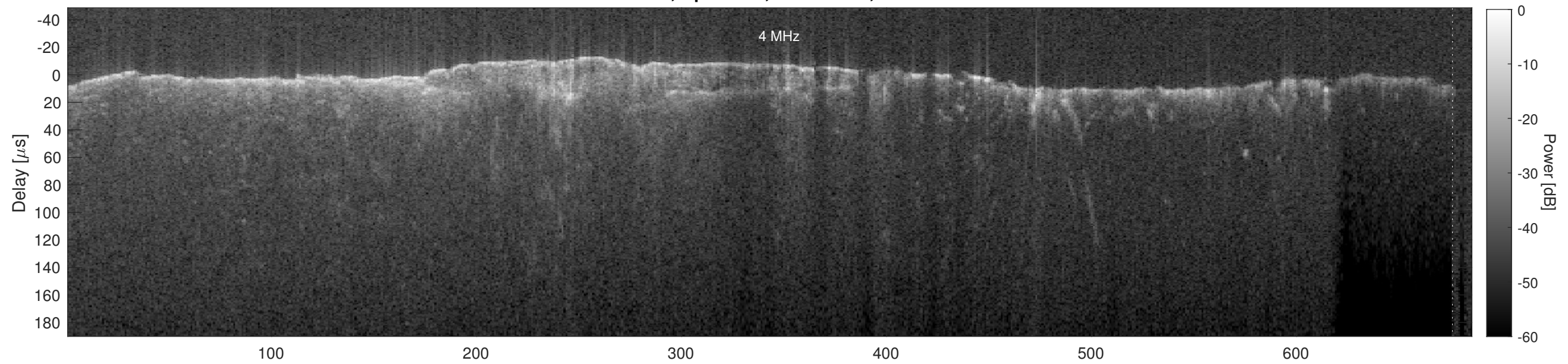
Orbit 16938, Cluttergram
