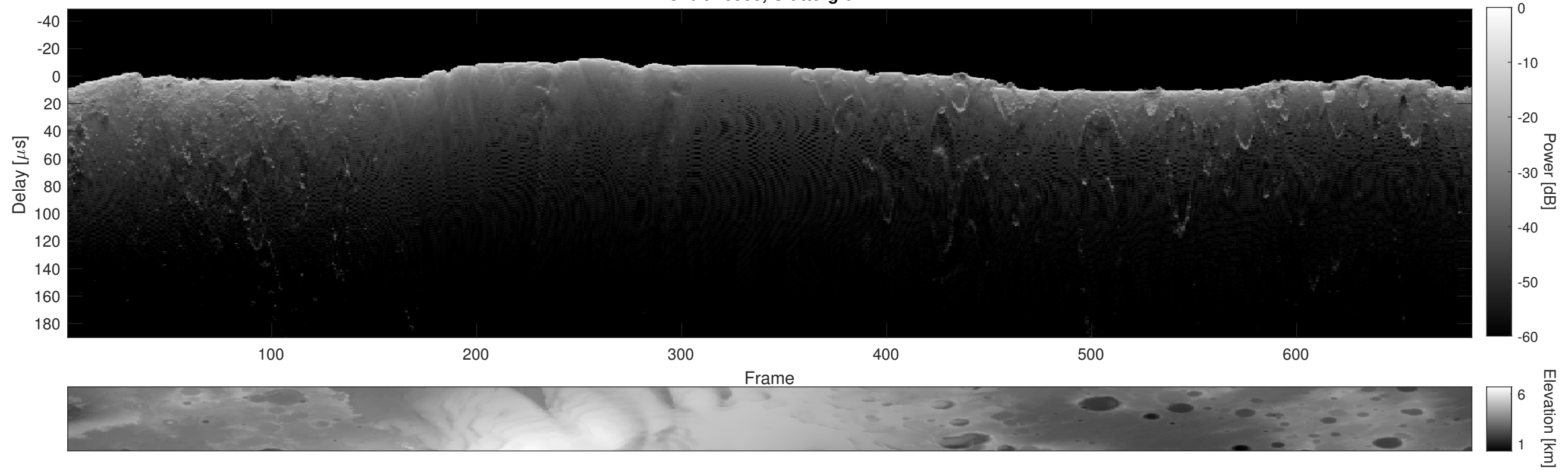
Orbit 16938, Cluttergram
