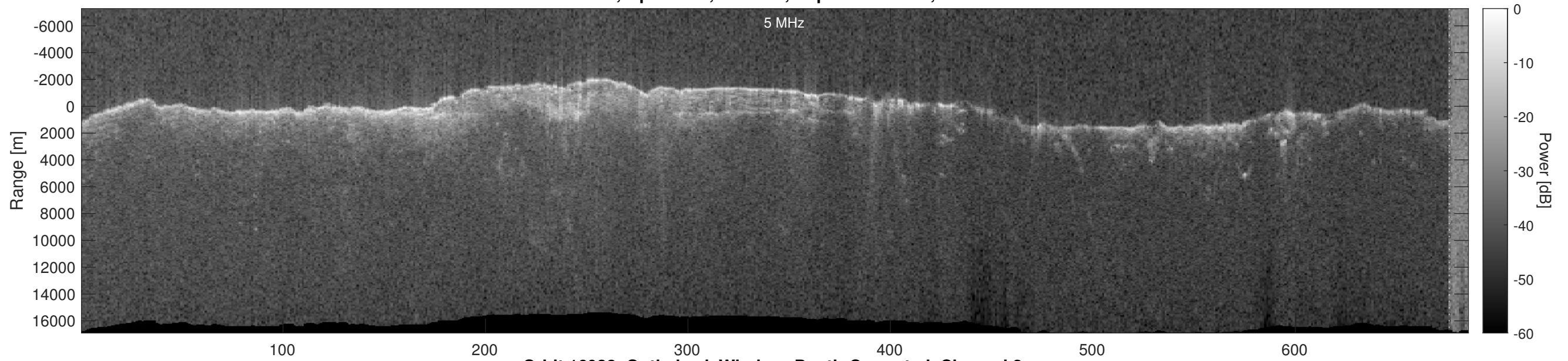
Orbit 16938, Optimized, Window, Depth-Corrected, Channel 2
