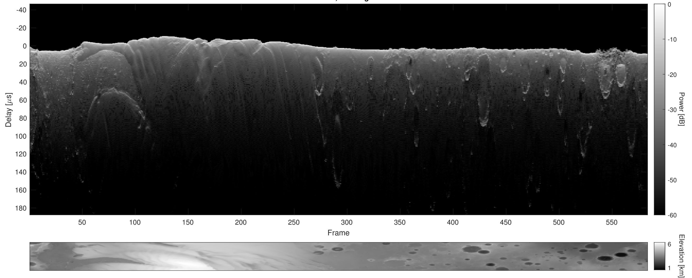
Orbit 16941, Cluttergram
