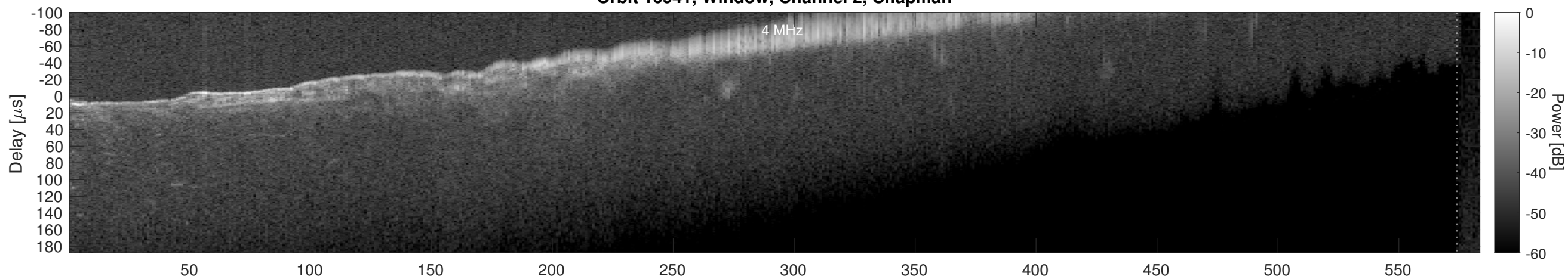
Orbit 16941, Window, Channel 2, Optimized
