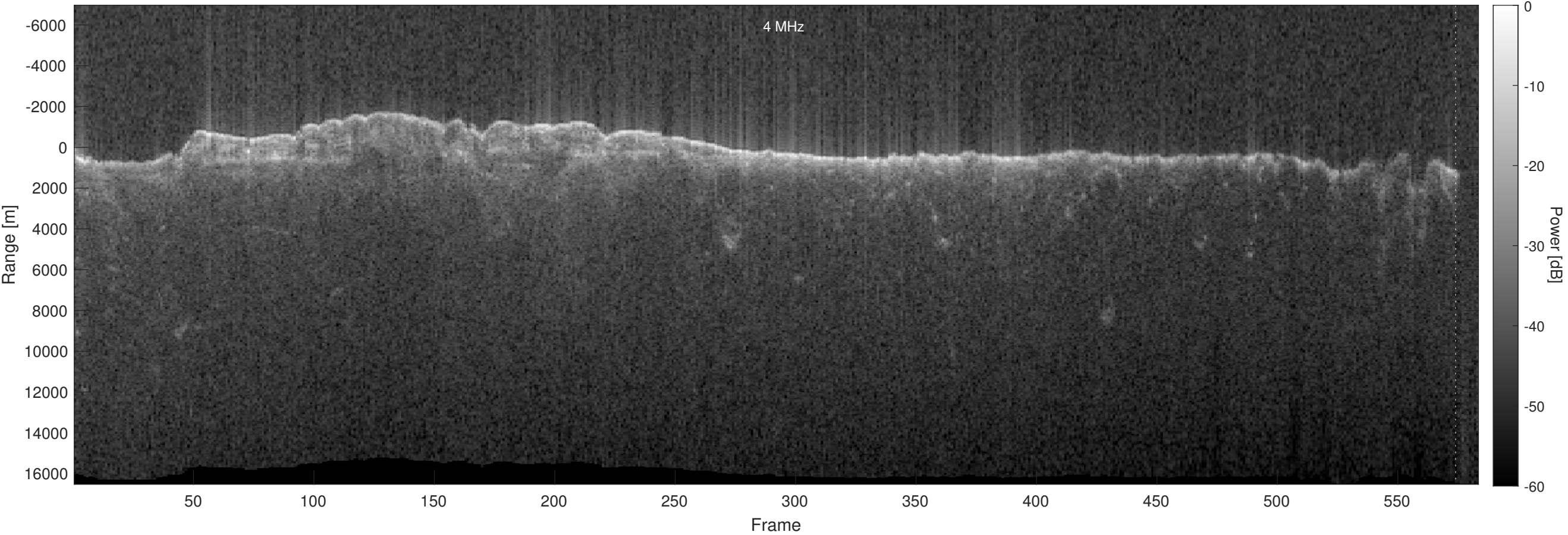
Orbit 16941, Optimized, No Window, Depth-Corrected, Channel 2
