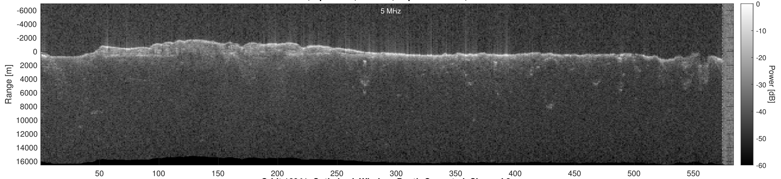
Orbit 16941, Optimized, Window, Depth-Corrected, Channel 2
