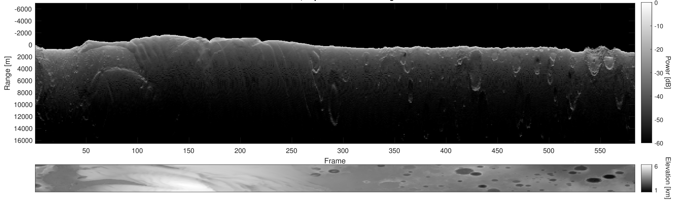
Orbit 16941, Depth-Corrected Cluttergram
