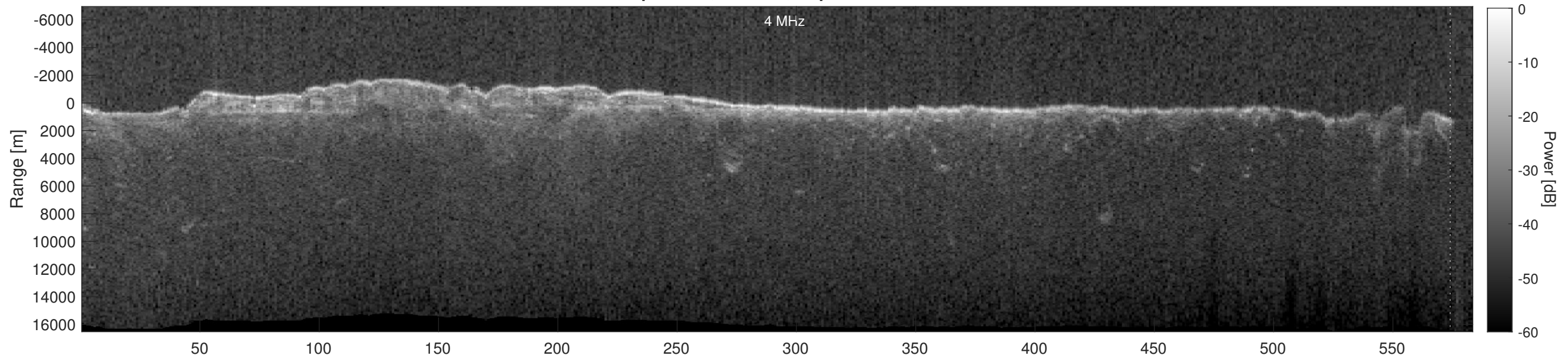
Orbit 16941, Depth-Corrected Cluttergram
