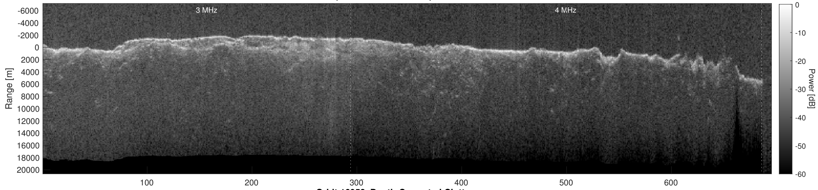
Orbit 16958, Depth-Corrected Cluttergram
