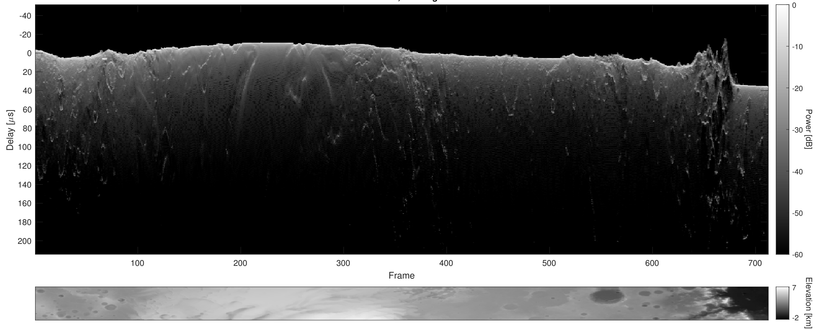
Orbit 16972, Cluttergram
