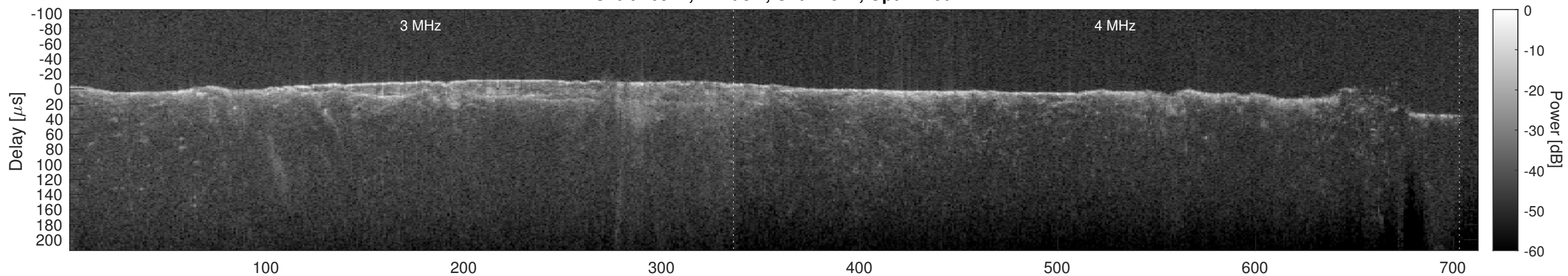
Orbit 16972, Cluttergram
