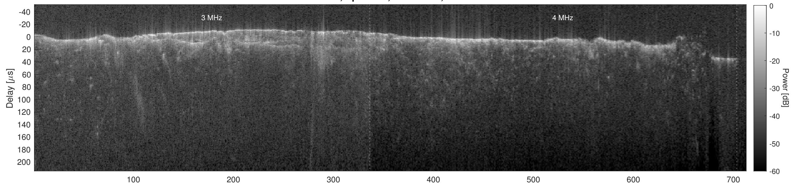
Orbit 16972, Cluttergram
