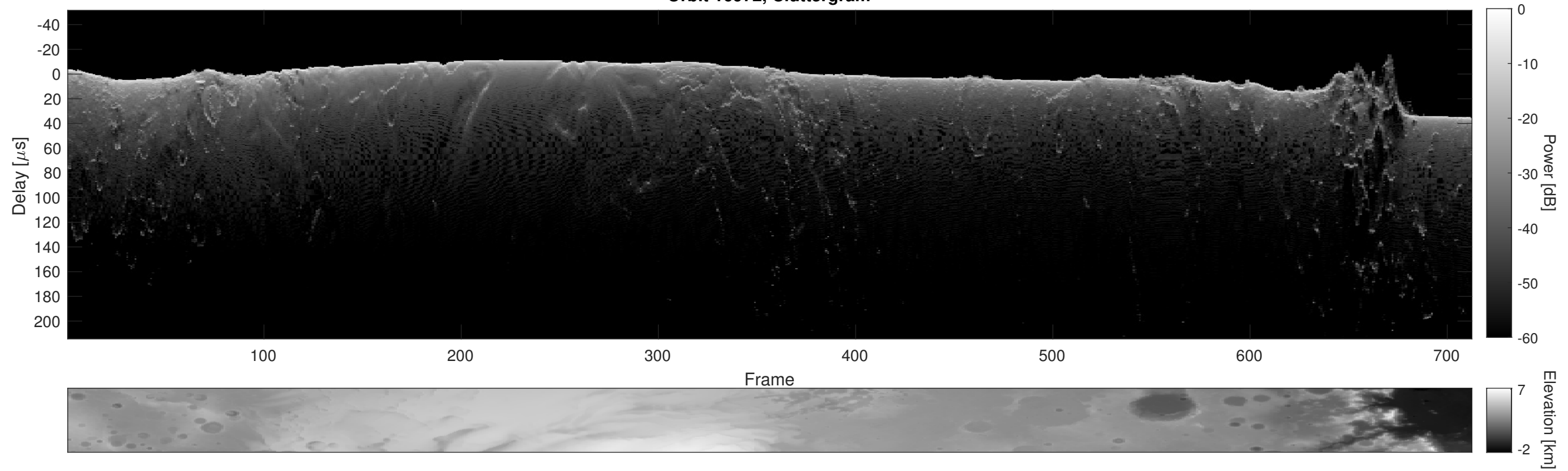
Orbit 16972, Cluttergram
