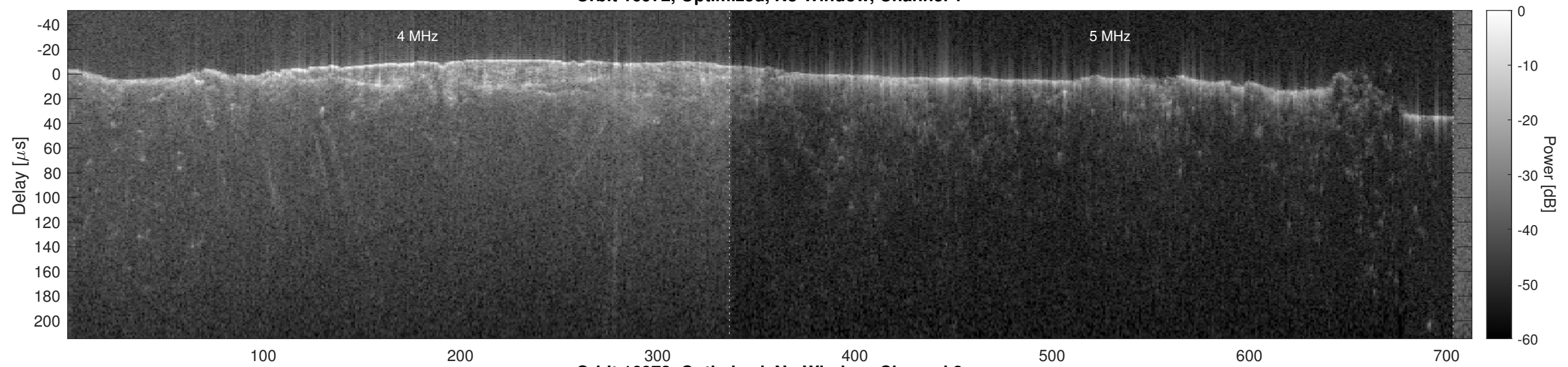
Orbit 16972, Optimized, No Window, Channel 2
