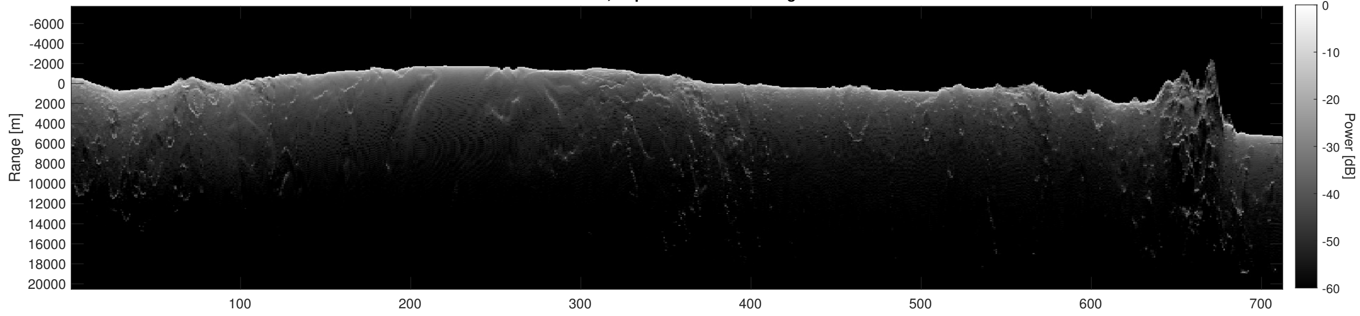
Orbit 16972, Depth-Corrected Cluttergram
