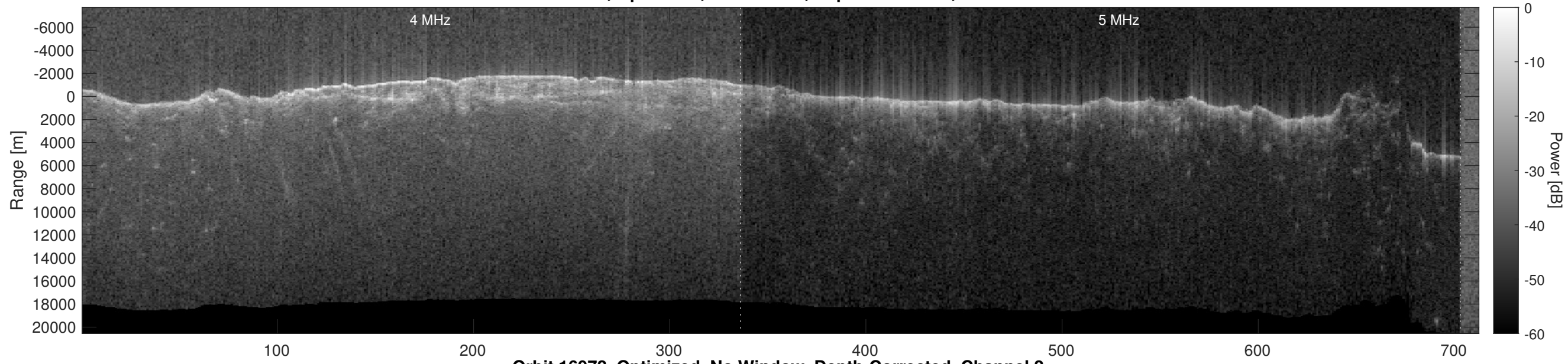
Orbit 16972, Optimized, No Window, Depth-Corrected, Channel 2
