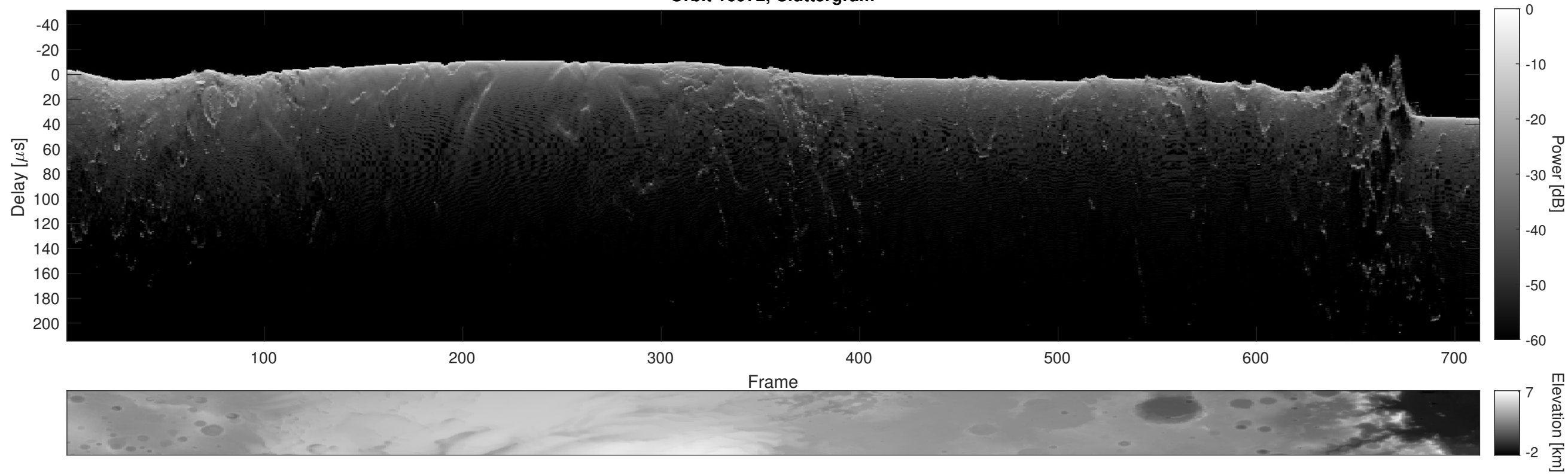
Orbit 16972, Cluttergram
