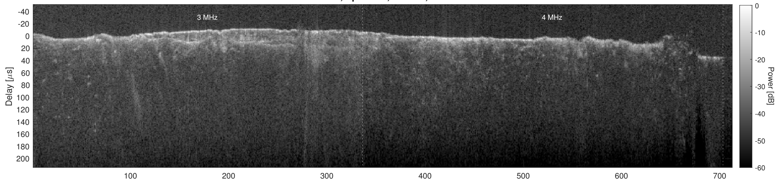
Orbit 16972, Cluttergram
