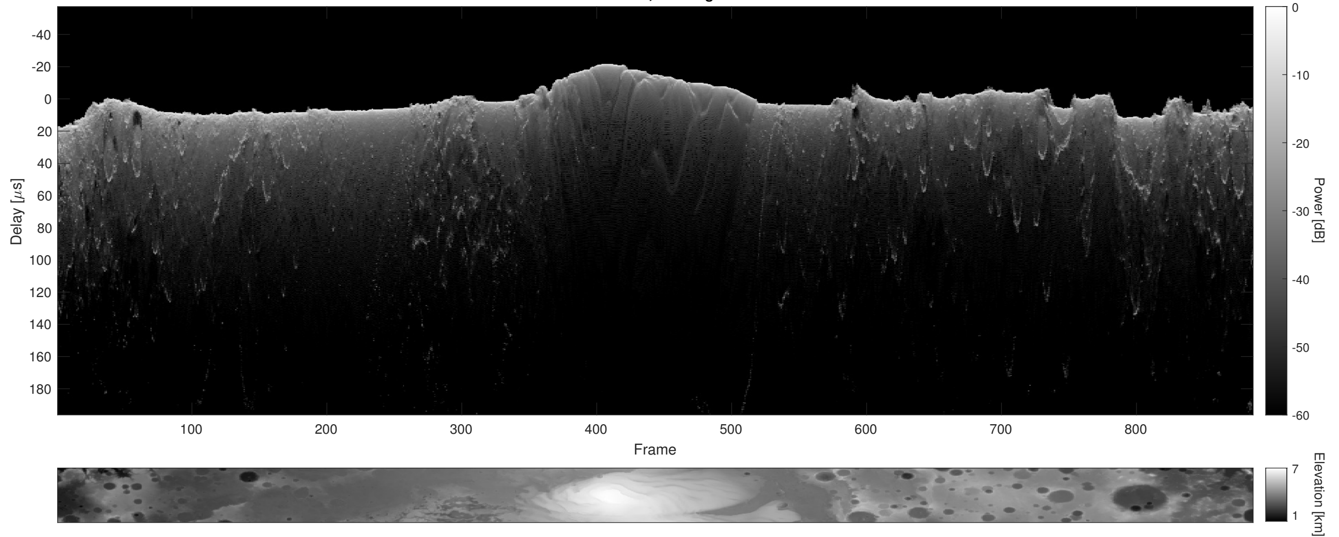
Orbit 17041, Cluttergram
