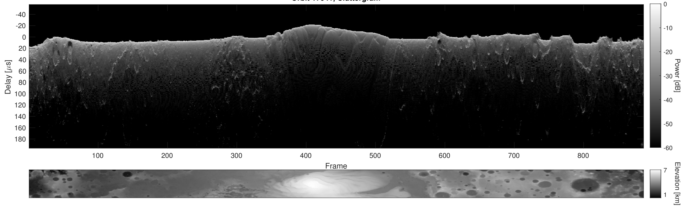
Orbit 17041, Cluttergram
