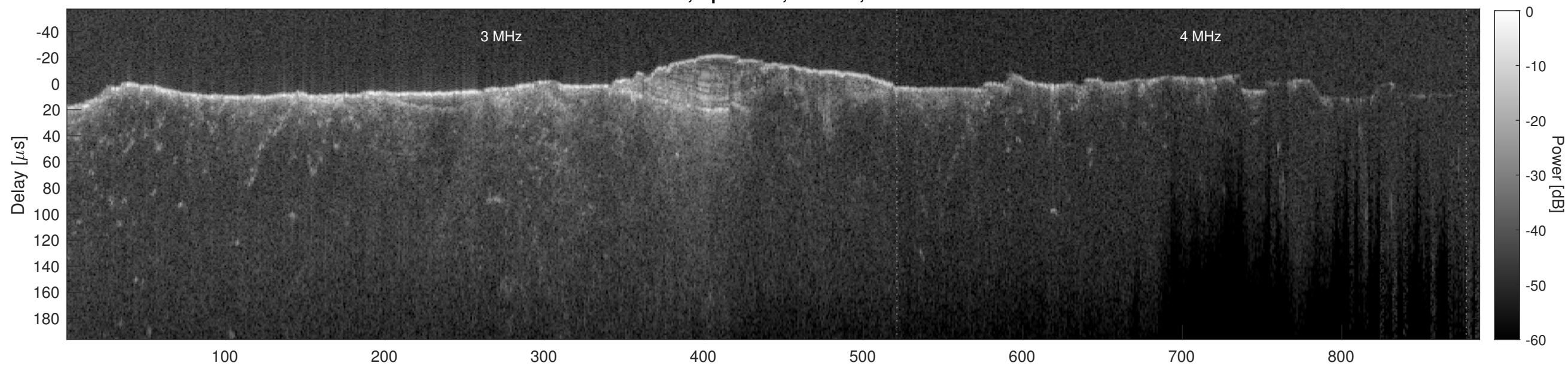
Orbit 17041, Cluttergram
