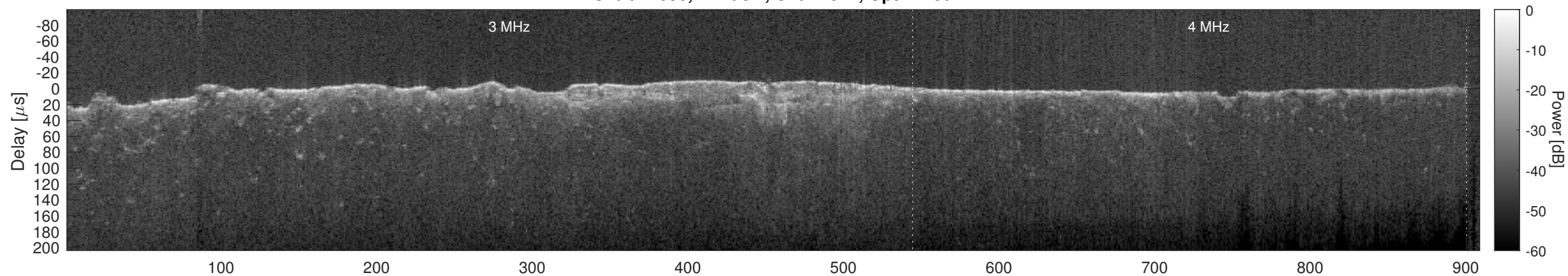
Orbit 17050, Cluttergram
