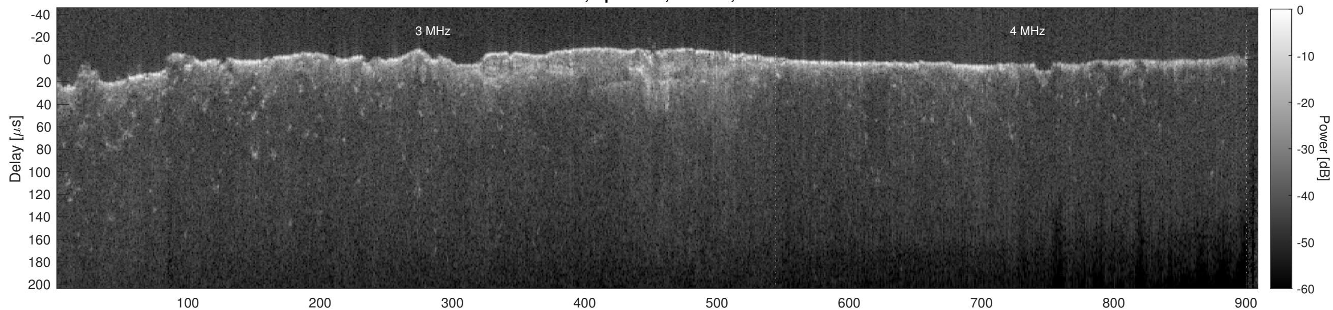
Orbit 17050, Cluttergram
