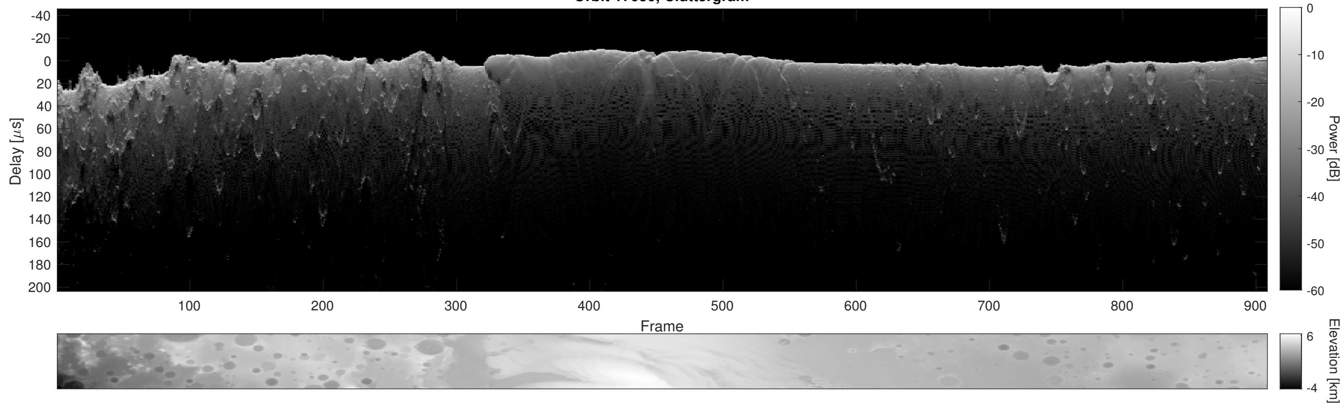
Orbit 17050, Cluttergram
