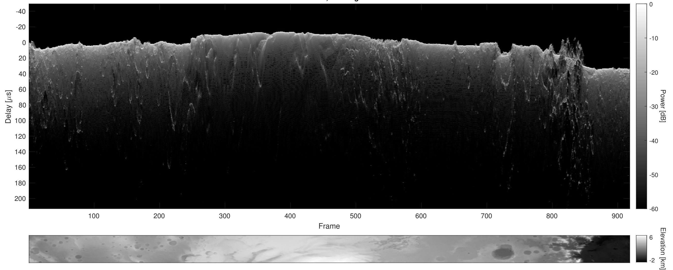
Orbit 17053, Cluttergram
