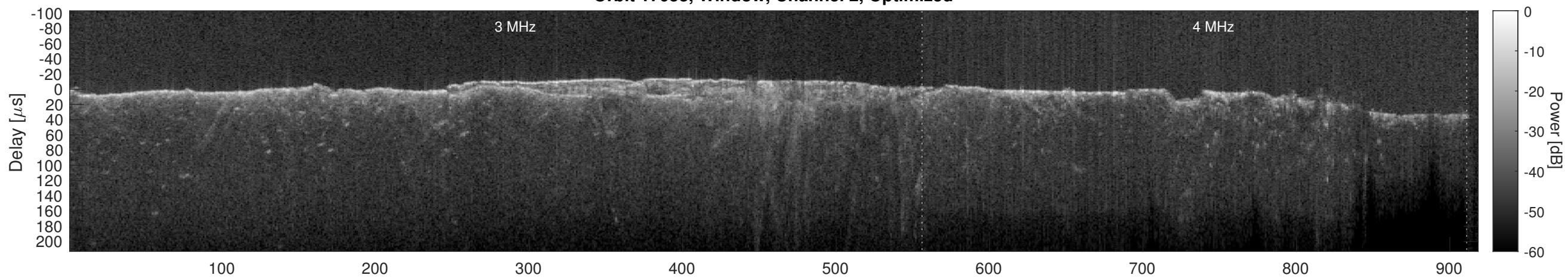
Orbit 17053, Cluttergram
