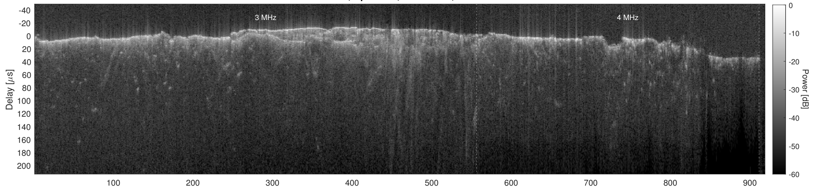
Orbit 17053, Cluttergram
