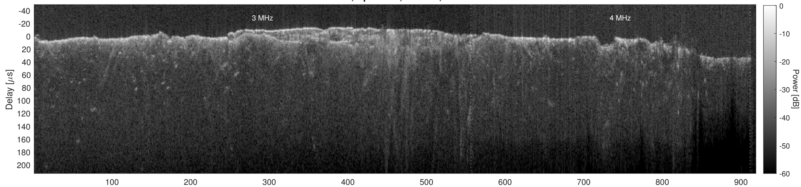
Orbit 17053, Cluttergram
