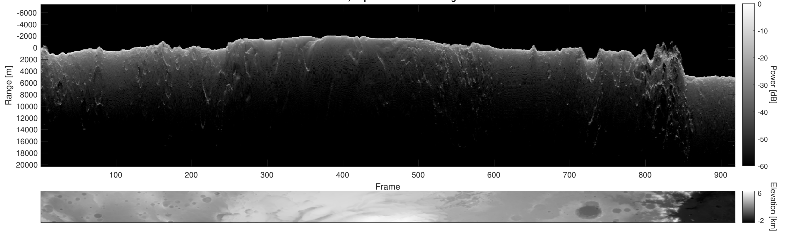
Orbit 17053, Depth-Corrected Cluttergram
