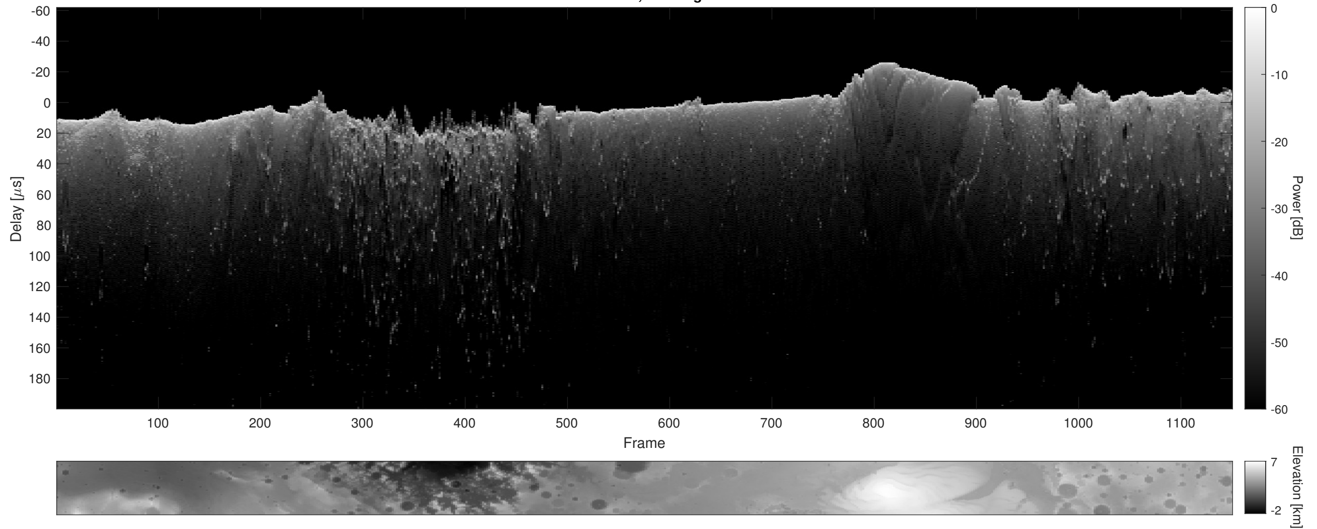
Orbit 17245, Cluttergram
