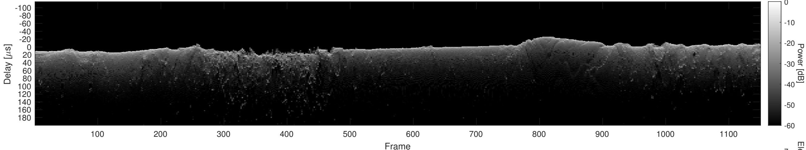
Orbit 17245, Cluttergram
