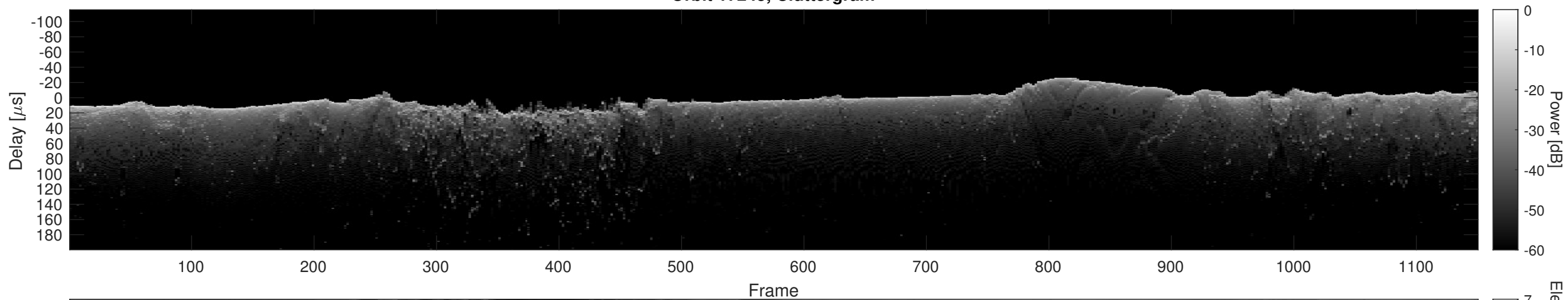
Orbit 17245, Cluttergram
