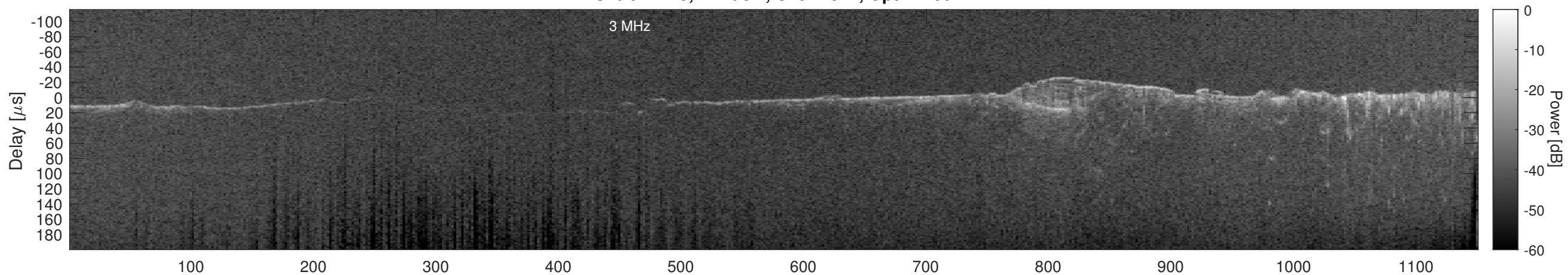
Orbit 17245, Cluttergram
