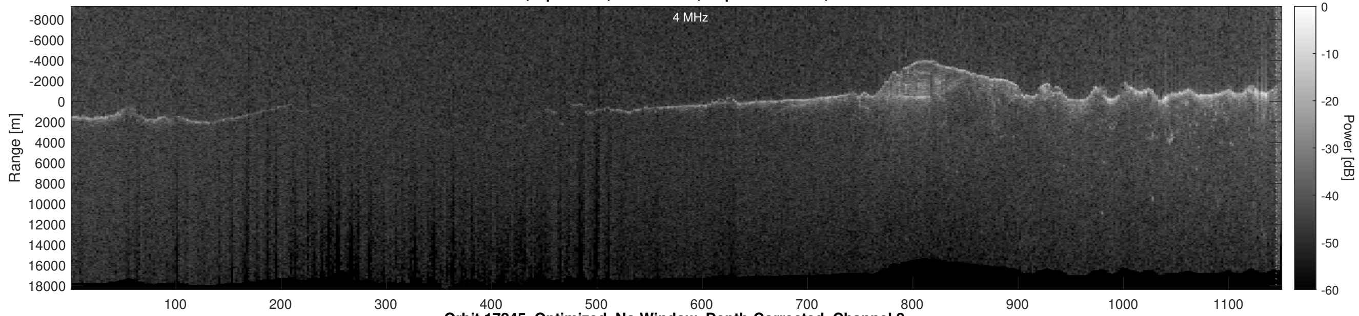
Orbit 17245, Optimized, No Window, Depth-Corrected, Channel 2
