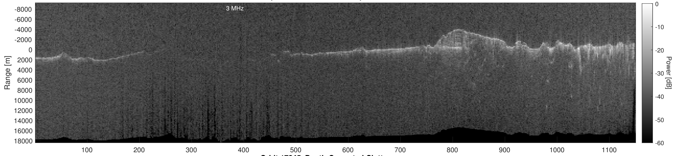
Orbit 17245, Depth-Corrected Cluttergram
