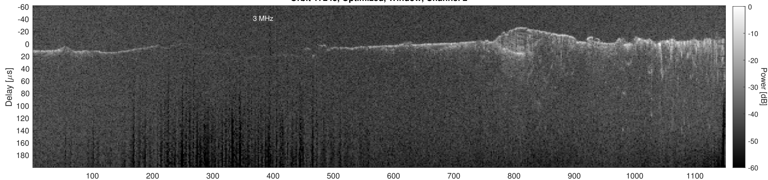
Orbit 17245, Cluttergram
