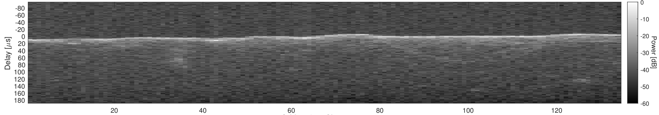
Orbit 17255, Cluttergram
