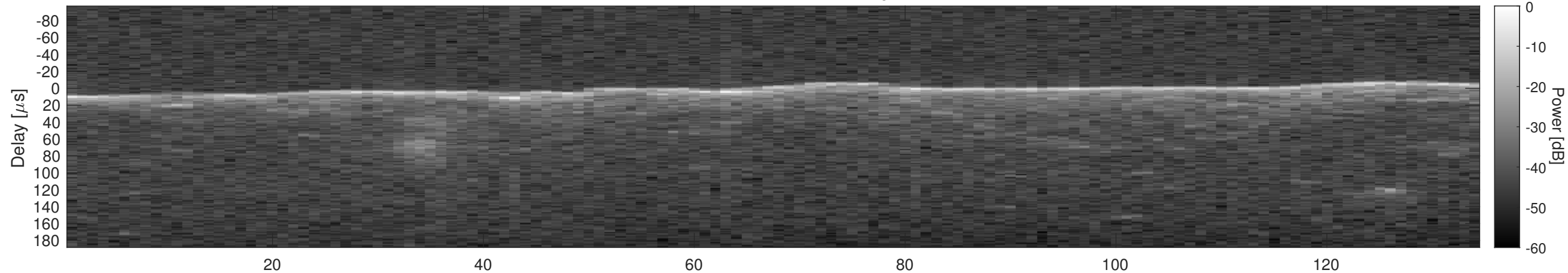
Orbit 17255, Cluttergram
