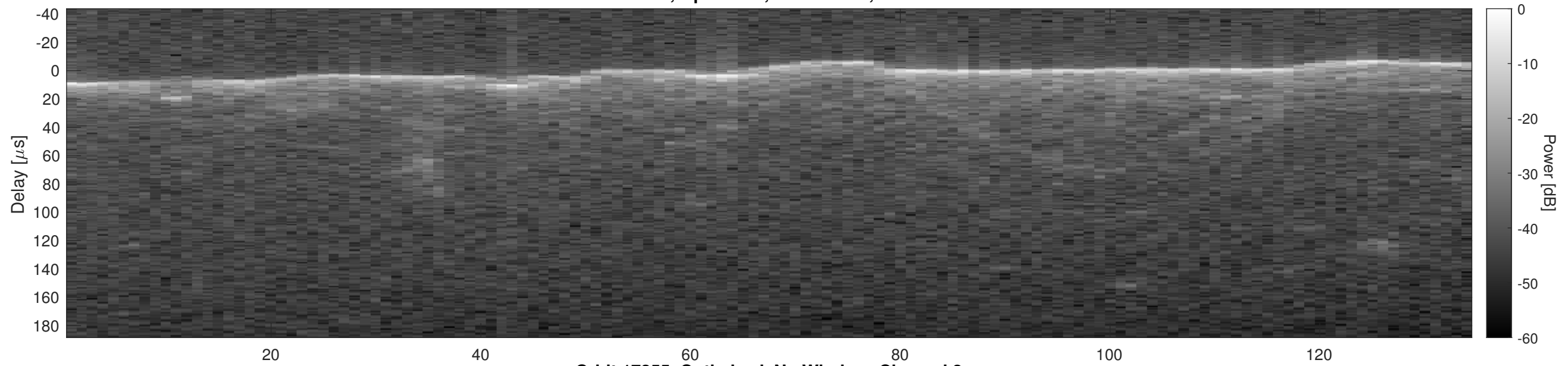
Orbit 17255, Optimized, No Window, Channel 2
