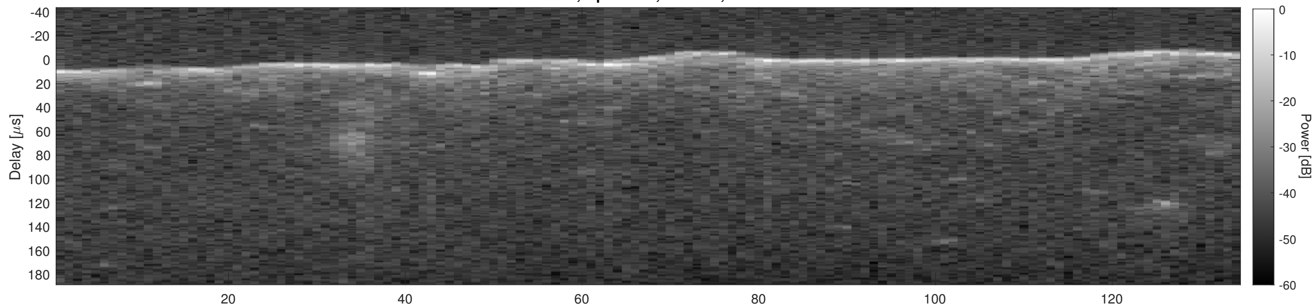
Orbit 17255, Cluttergram
