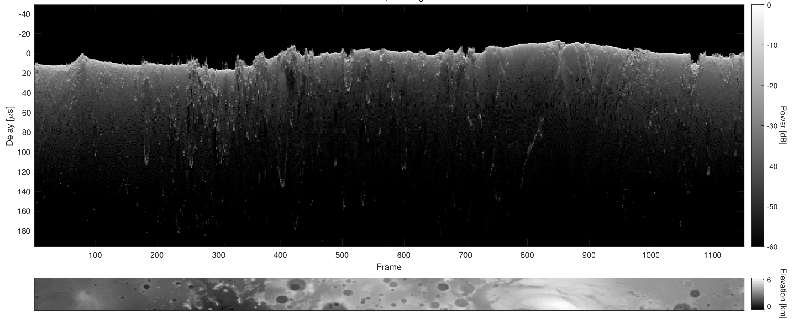
Orbit 17261, Cluttergram
