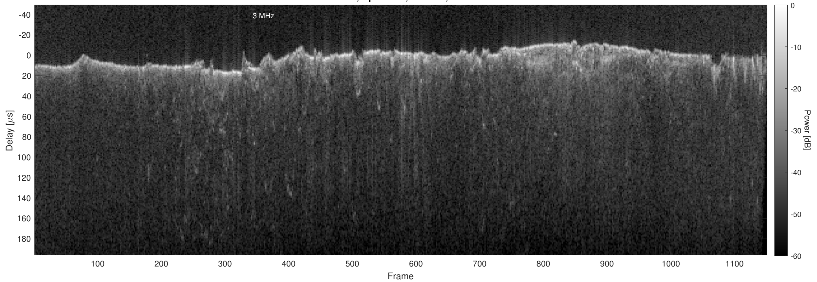
Orbit 17261, Optimized, Window, Channel 2
