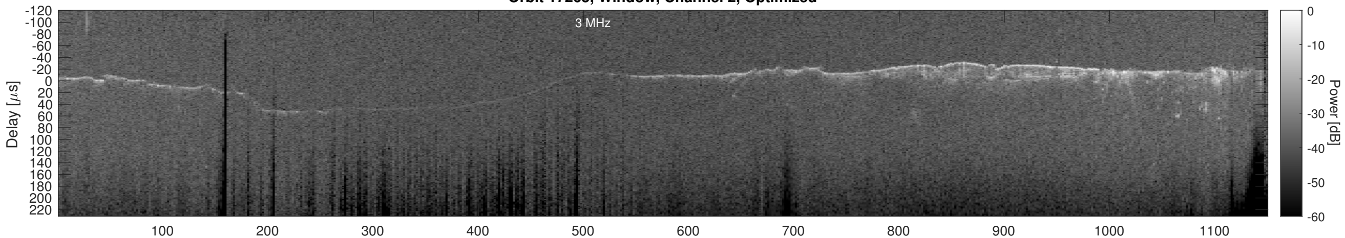
Orbit 17265, Cluttergram
