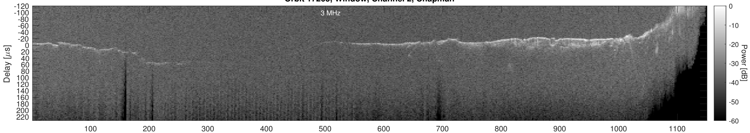
Orbit 17265, Window, Channel 2, Optimized
