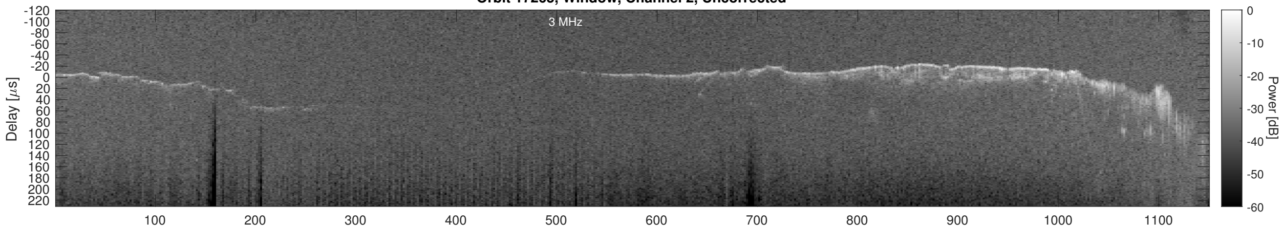
Orbit 17265, Window, Channel 2, Chapman
