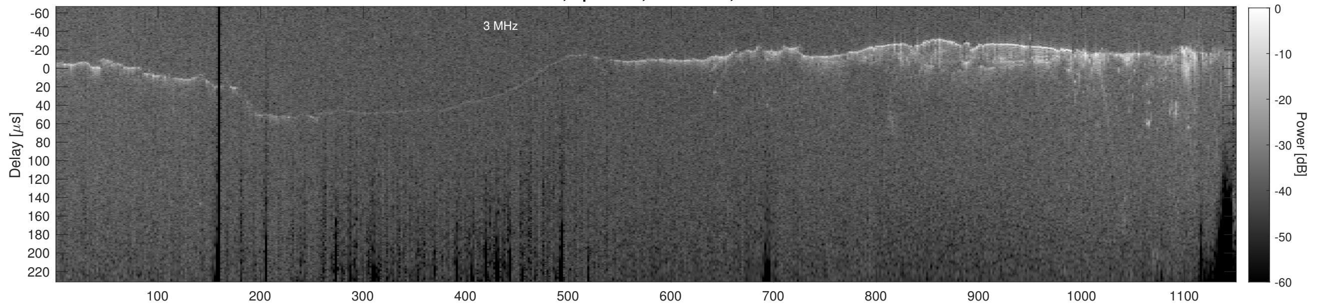
Orbit 17265, Cluttergram
