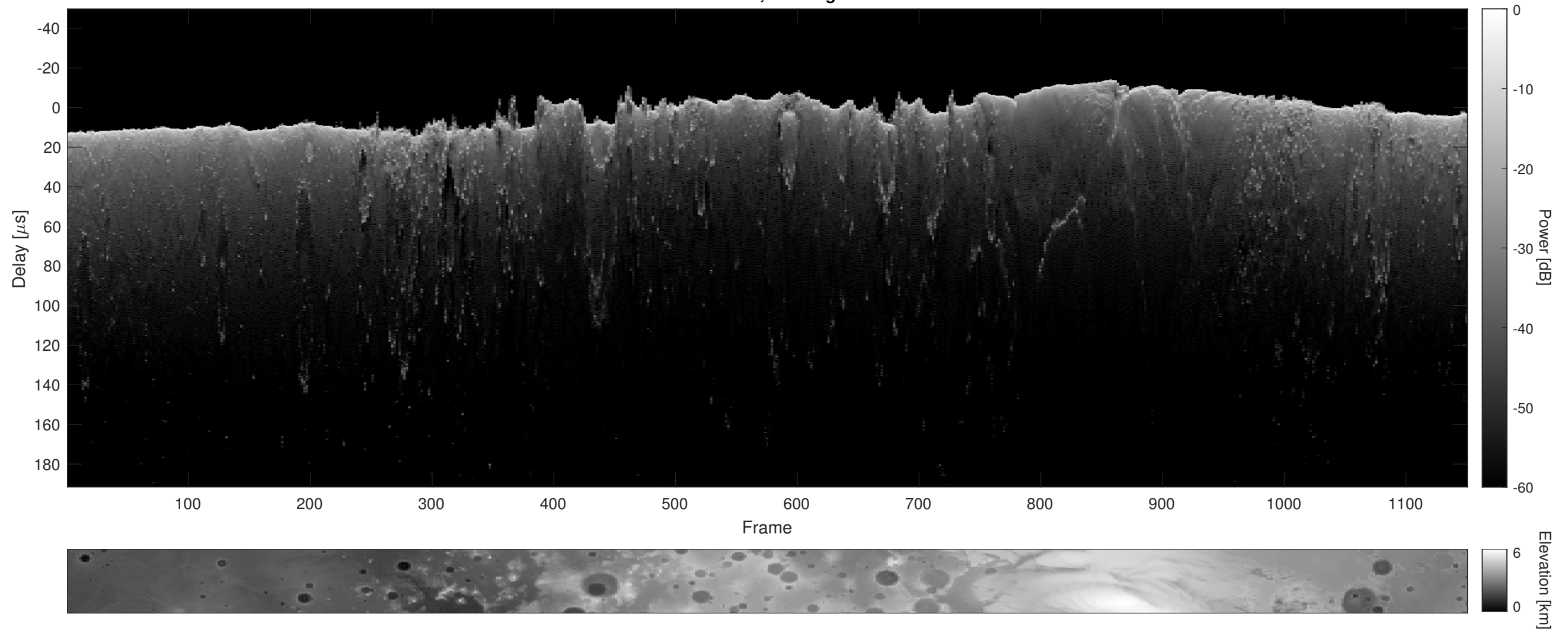
Orbit 17268, Cluttergram
